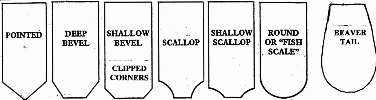
SHAPES OF ROOF SLATES
